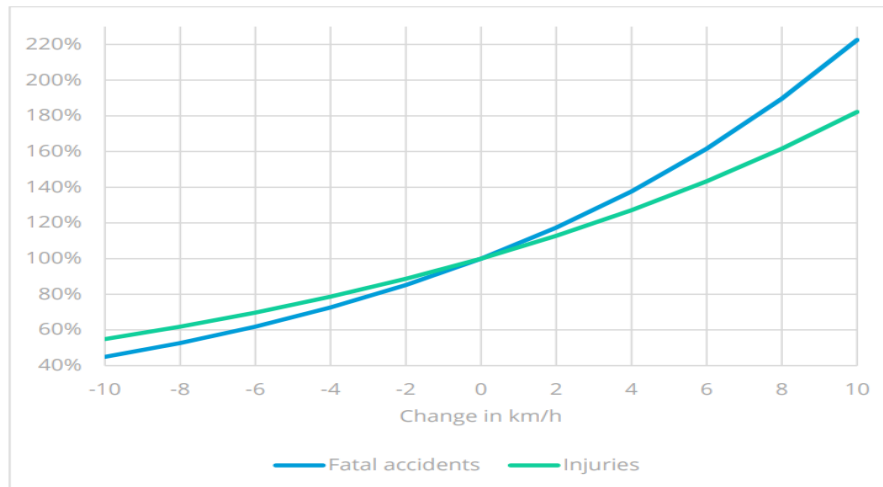
Figure 1. Relationship between speed change and crash rate Source: Van den Berghe & Pelssers (2020) based on coefficients of exponential model in Elvik et al. (2019)
